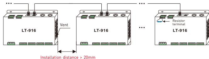
RJ45 connected in parallel
