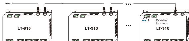
3-pin XLR connected in parallel
